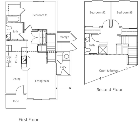
3 - Bedroom Townhouse Floor Plan
